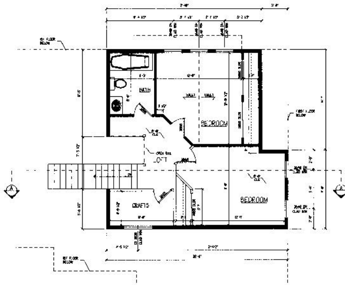
SECOND FLOOR PLAN SQUARE FOOTAGE: 567 SF
