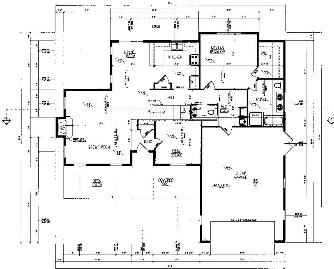
FIRST FLOOR PLAN SQUARE FOOTAGE: 358 SF
